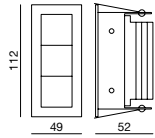
CEILING CUT 105x40
